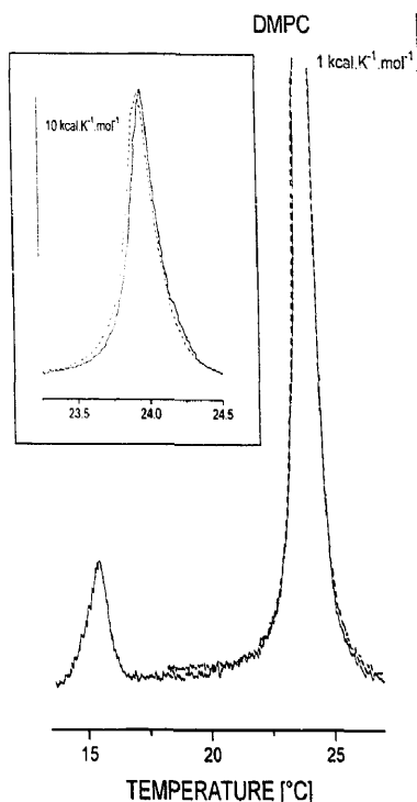
Fig. 1. DSC heating thermograms (in two different Y-scales) of hydrated DMPC dispersion recorded after cooling from 28°C to 10°C (full line) and to 17°C (dashed line). Heating rate 0.5 K/min.
