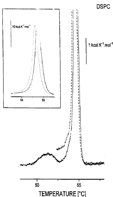
Fig. 3. DSC heating thermograms (in two different Y-scales) of hydrated DSPC dispersion recorded after cooling from 58°C to 30°C (full line) and to 51°C (dashed line). Heating rate 0.5 K/min.
