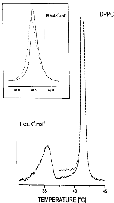
Fig. 2. DSC heating thermograms (in two different Y-scales) of hydrated DPPC dispersion recorded after cooling from 45°C to 20°C (full line) and to 35°C (dashed line). Heating rate 0.5 K/min.
