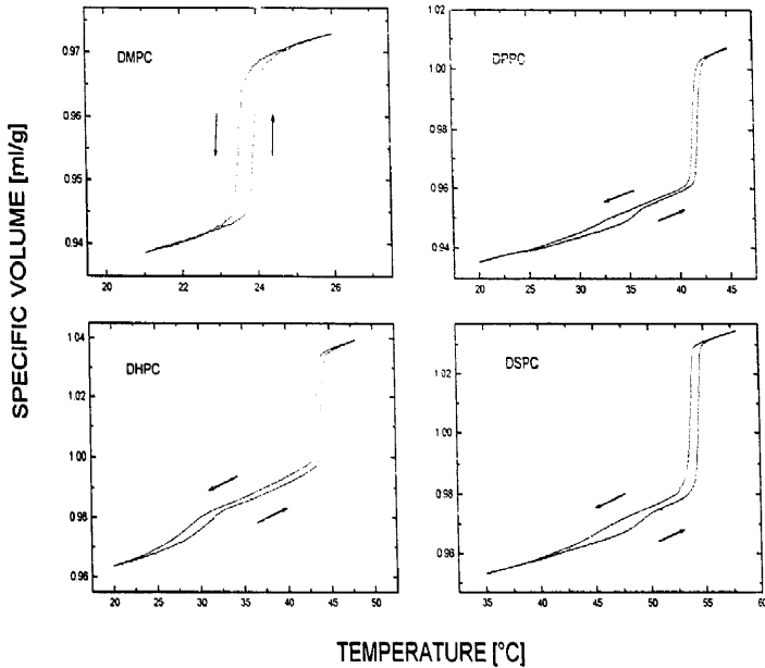
Fig. 5. Densitometric heating and cooling traces of hydrated DMPC, DPPC, DSPC, and DHPC dispersions recorded at a scan rate of 0.5 K/min.
