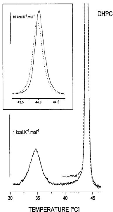
Fig. 4. DSC heating thermograms (in two different Y-scales) of hydrated DHPC dispersion recorded after cooling from 48°C to 20°C (full line) and to 38°C (dashed line). Heating rate 0.5 K/min.
