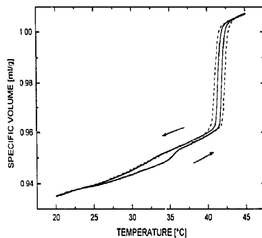
Fig. 6. Densitometric heating and cooling traces of hydrated DPPC dispersion recorded at scan rate of 0.1 K/min (full line) and 1 K/min (dashed line).
